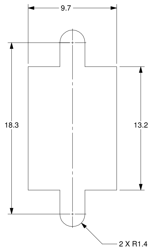
RECOMMENDED PANEL HOLE
