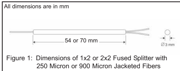
Fused Splitter With 3 mm Cable
